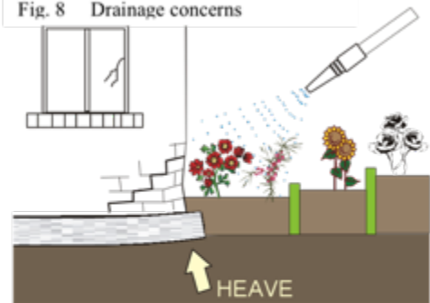
Fig. 8 Drainage concerns
